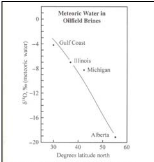
FIGURE 26.15 Latitude dependence of the \delta^{18}\text{O} values of the intersections of the brine arrays with the meteoric-water line in Figure 26.14. Based on data of Clayton et al. (1966).
